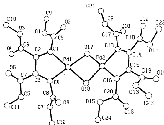
Figure 1. X-ray single-crystal structure of 1
