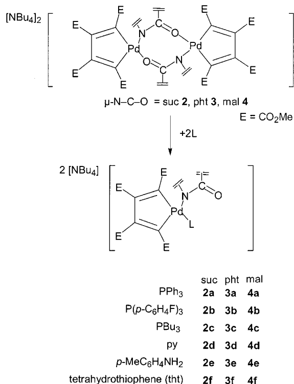
Scheme 2. Mononuclear N -imidate complexes
