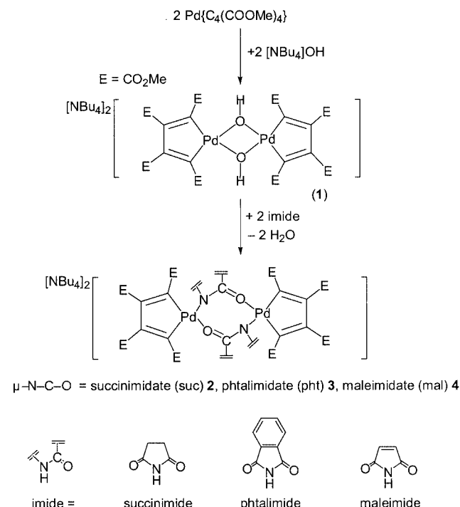
Scheme 1. Hydroxo- and imideate-bridged binuclear complexes
