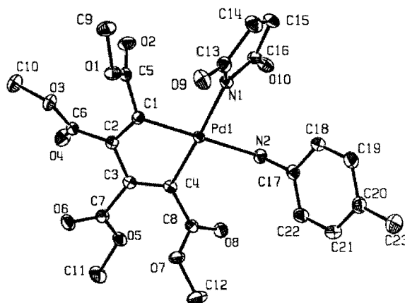
Figure 3. X-ray single crystal structure of 4e
