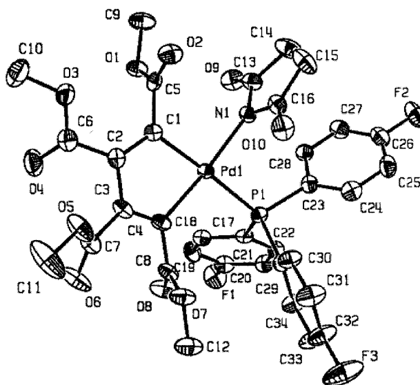
Figure 2. X-ray single crystal structure of 4b
